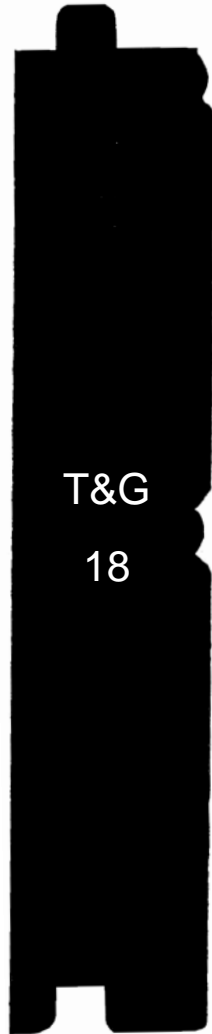
T&G-18 1" x 5 3/8"
